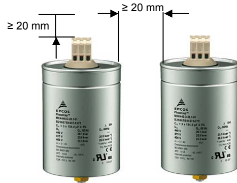
Fig. 3: Minimum distance between PFC capacitors of the PhaseCap series
