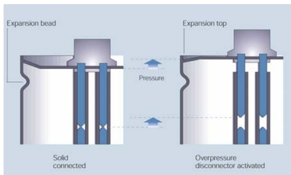
Fig. 4: Overpressure disconnector
