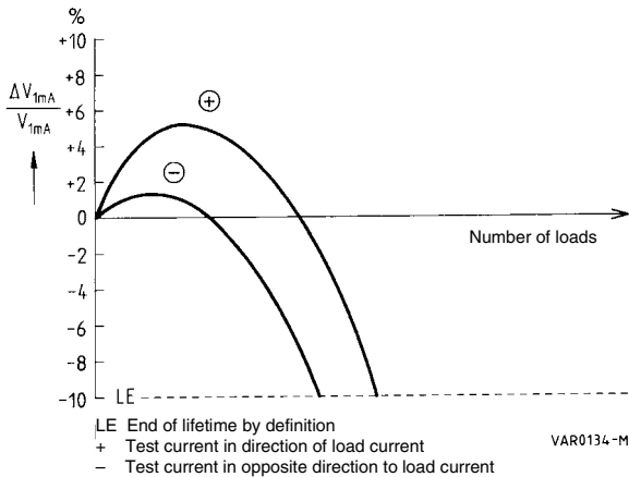
Figure 24 Typical polarization effect for unipolar loading of metal oxide varistors
