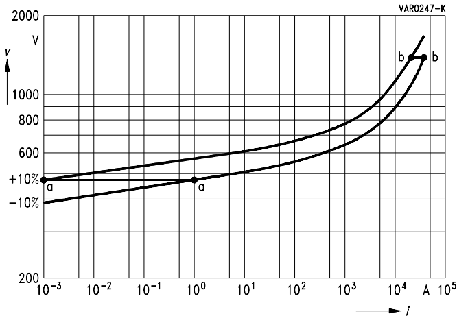
Figure 18 Tolerance band of the SIOV-B40K275
