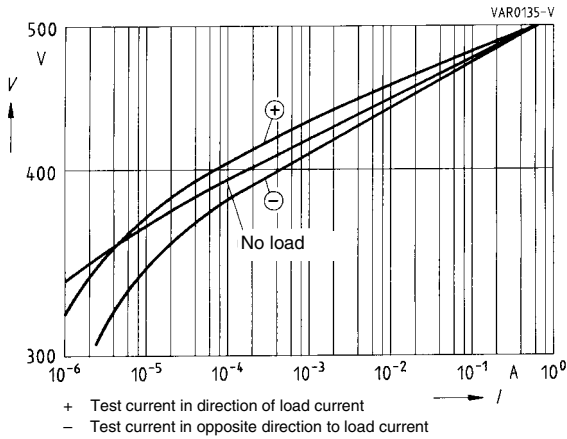
Figure 25 Typical polarization effects of leakage current for unipolar loading of metal oxide varistors
