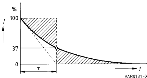
Figure 20 Time constant of fly-wheel circuit
