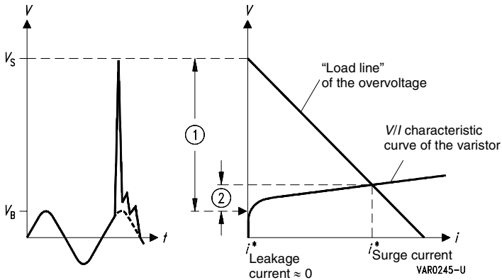
Figure 16 Principle of overvoltage protection by varistors
