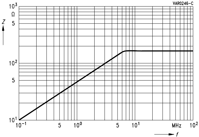
Figure 17 Impedance of a supply line for high-frequency overvoltages
