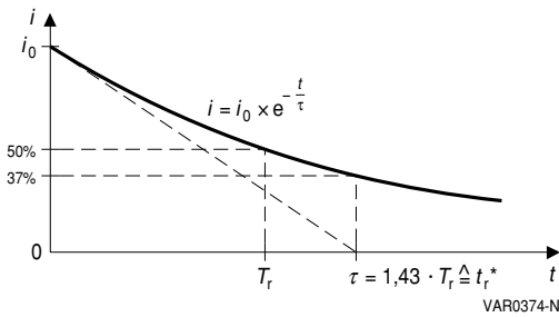
Figure 22 Equivalent rectangular wave of an e-function
