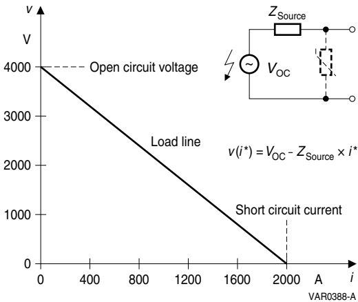
Figure 19a Load line in linear scale
