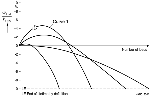
Figure 23 Typical curves for change in varistor voltage when metal oxide varistors are repeatedly loaded
