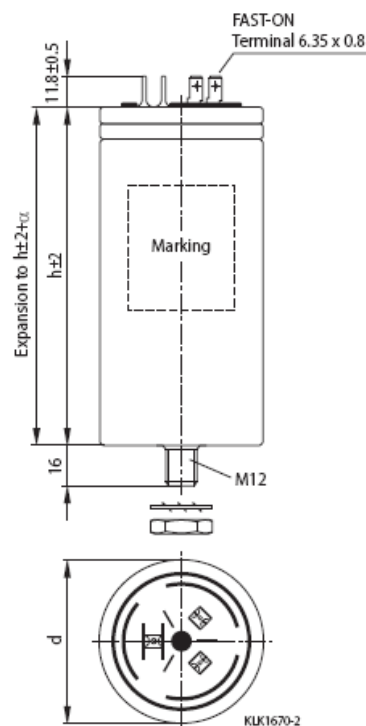
Dimensional drawing
