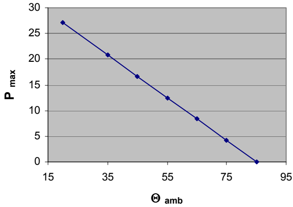
Max. allowable power loss at specific ambient Temp. B32344E5252A020
