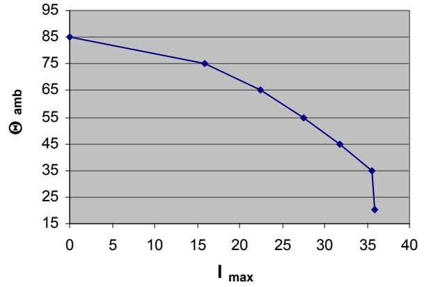
Max. allowable ambient Temp. at specific current (rms) B32344E5252A020
