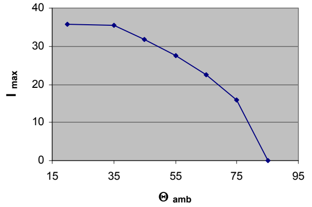
Max. allowable current (rms) at specific ambient Temp. B32344E5252A020
