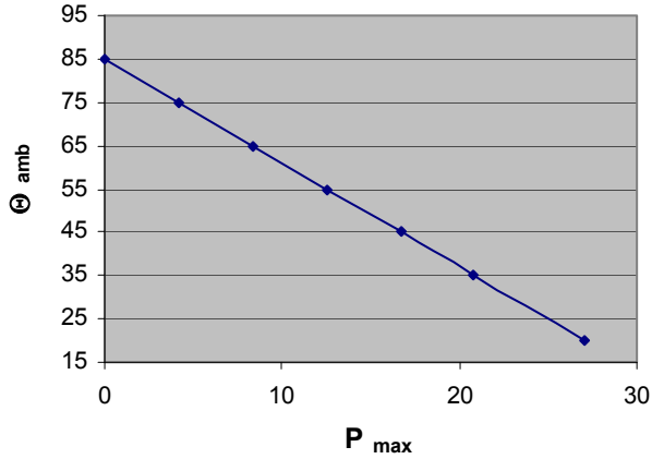
Max. allowable ambient Temp. at specific power loss B32344E5252A020
